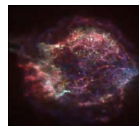
Cas A Distribution of Elements Animation
