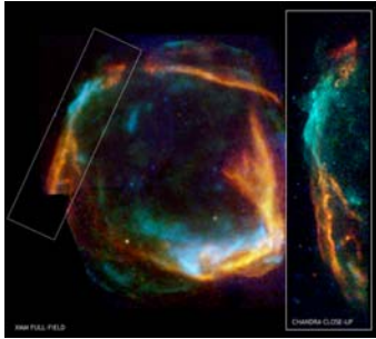
RCW 86 (Chandra, XMM-Newton)
